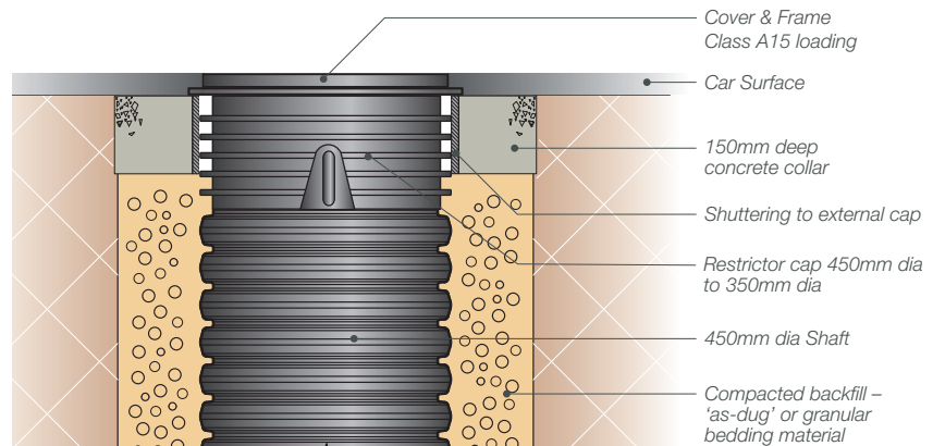
Fig. 32 – Installation detail A15 – domestic gardens and/or areas subject to occasional vehicle loading
