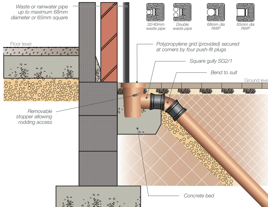
Fig. 22 – Square Gully SG2/1
