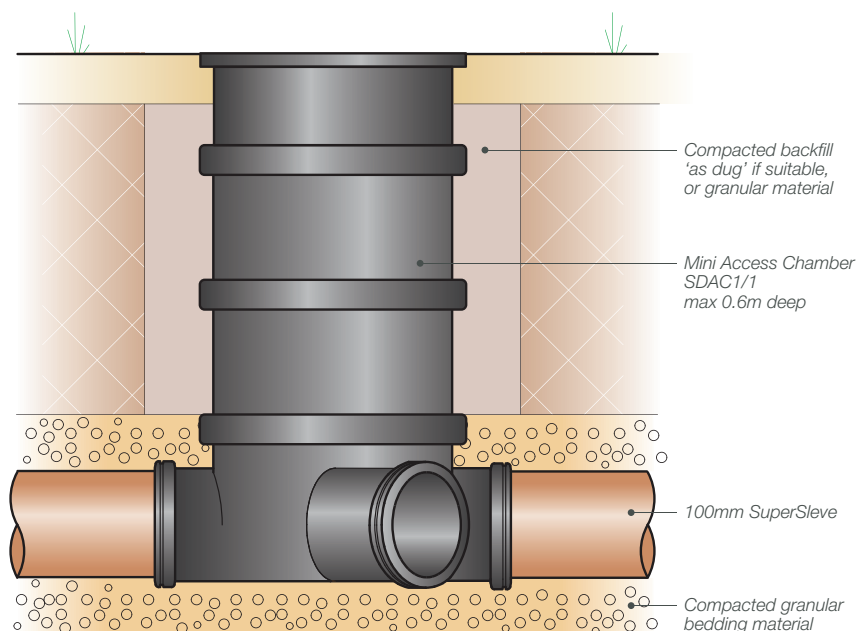
Fig. 26 – Installation detail – domestic gardens
