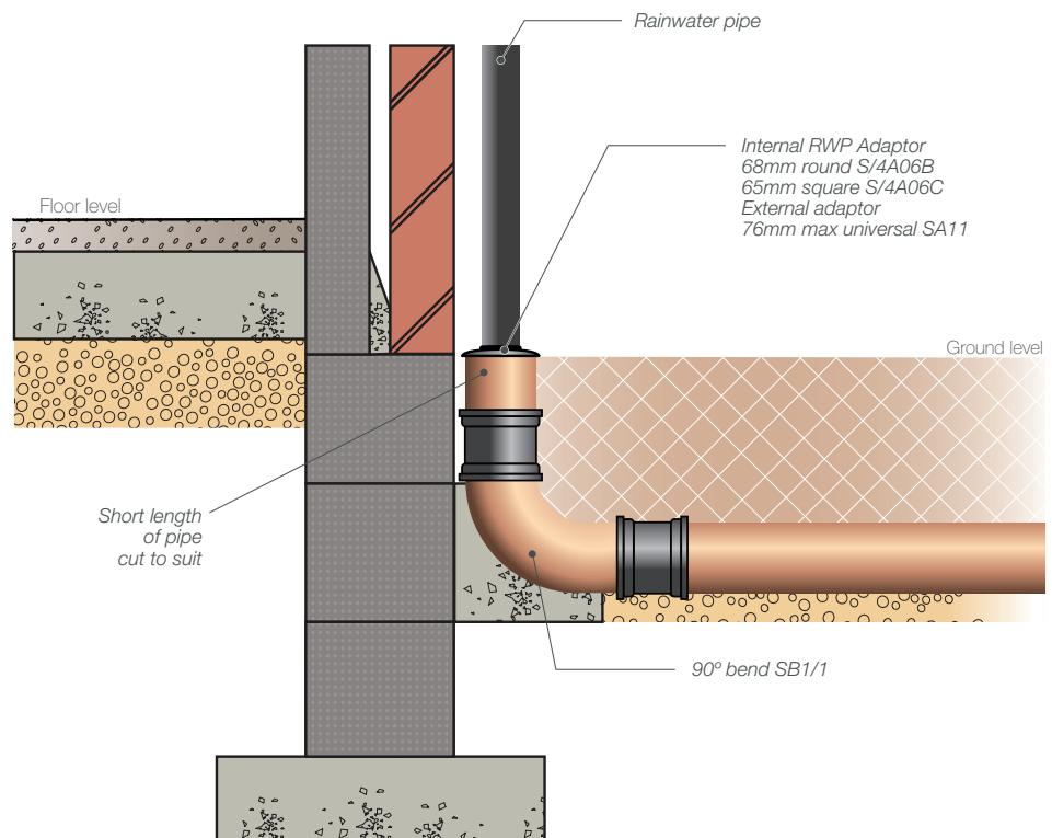
Fig. 16 – Connection of external rainwater pipe
