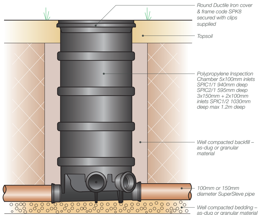
Fig. 28 – Installation detail – domestic gardens
