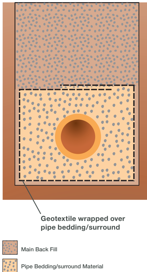
Fig. 7 – Use of Geotextile material around pipe bedding in waterlogged ground
