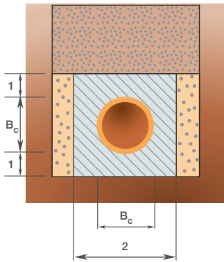
a. Unreinforced concrete surround. Bedding factor 4.5 (maximum diameter 600 mm). Reference: ASCE Gravity sanitary sewer design and construction [1]
