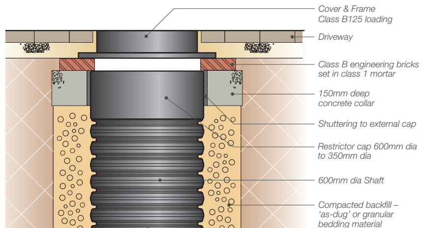
Fig. 36 – Installation detail B125 loading – paved areas with limited traffic load
