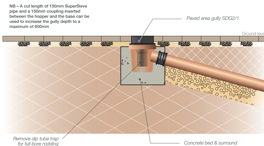
Fig. 23 – Paved Area Gully SDG2-1
