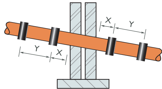
a. Pipe built-in to structure
