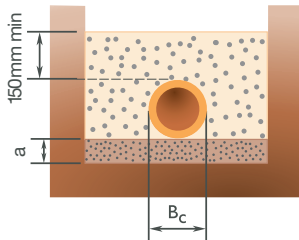
Class N Bedding Factor 1.1
