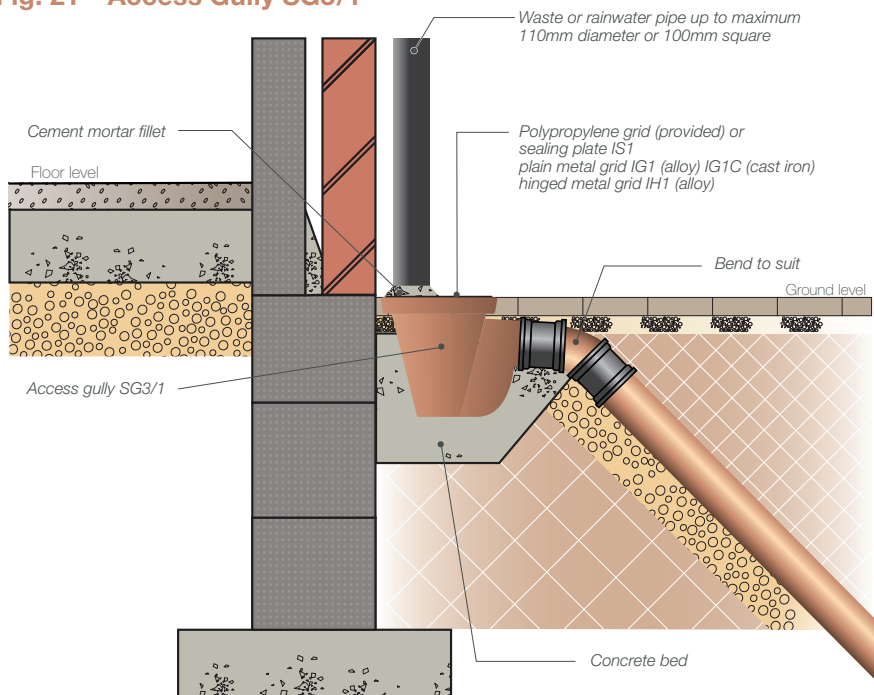
Fig. 21 – Access Gully SG3/1
