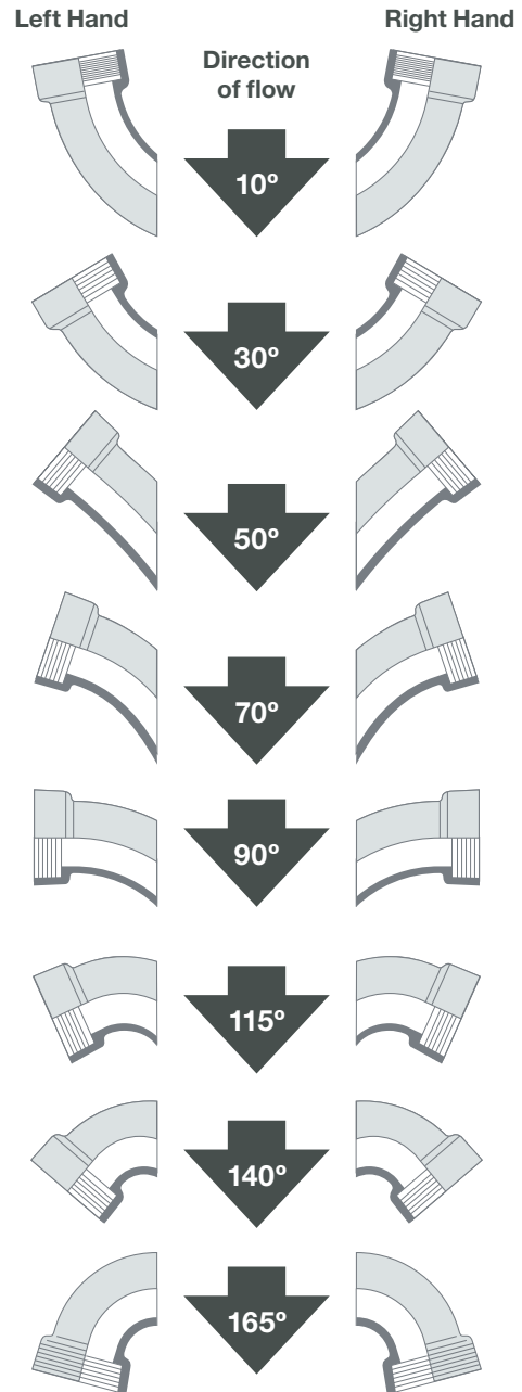
Fig. 38 – Branch channel bend selector (for half section and 3/4 section)
