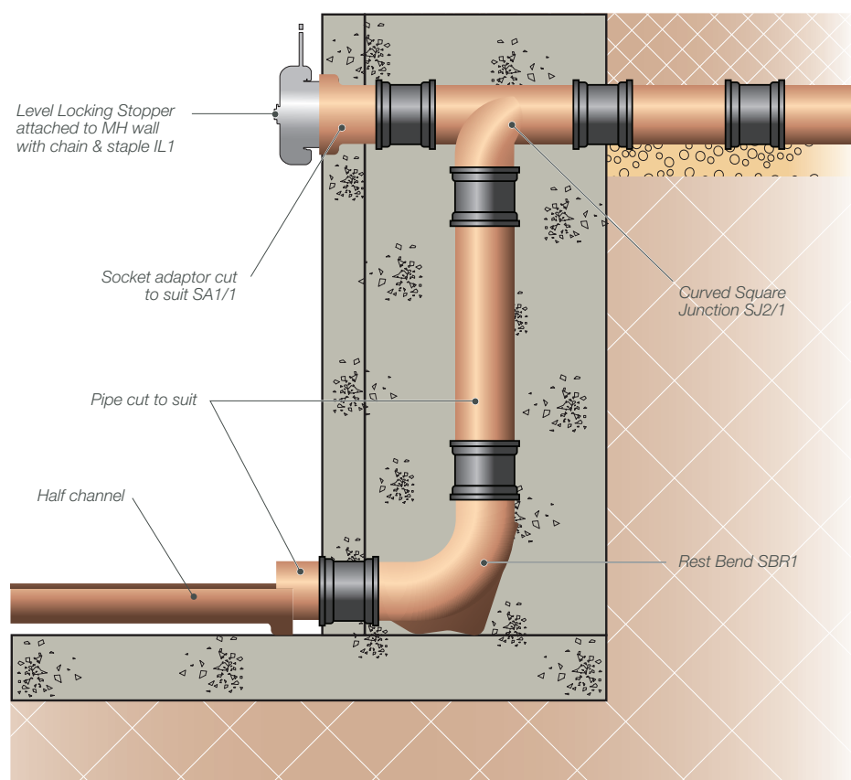
Fig. 39 – Backdrop connections
