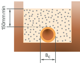
Class D Bedding Factor 1.1
