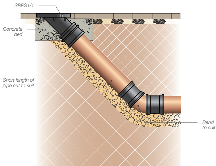
Fig. 25 – Square Top Rodding Point
