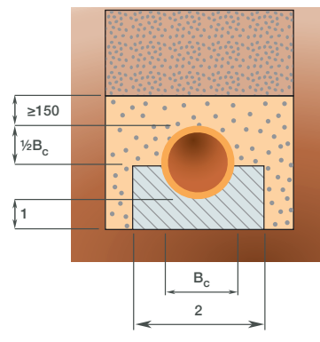
d. Unreinforced concrete bed. Bedding factor 2.6
