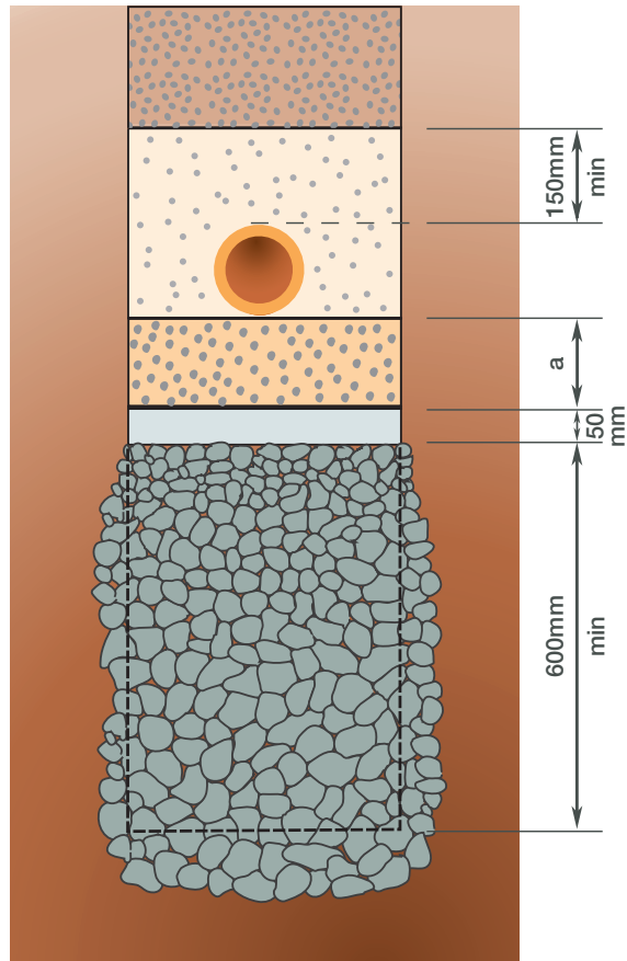
Fig. 6 – Class F bedding construction in soft ground
