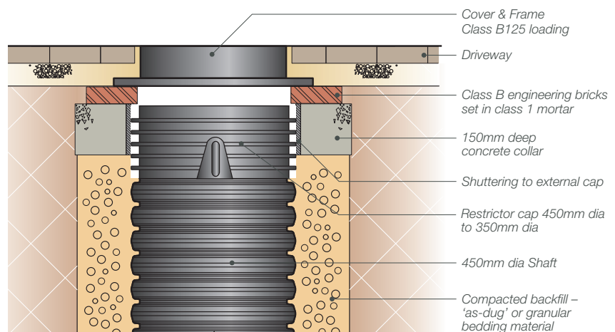
Fig. 33 – Installation detail B125 loading – paved areas with limited traffic load
