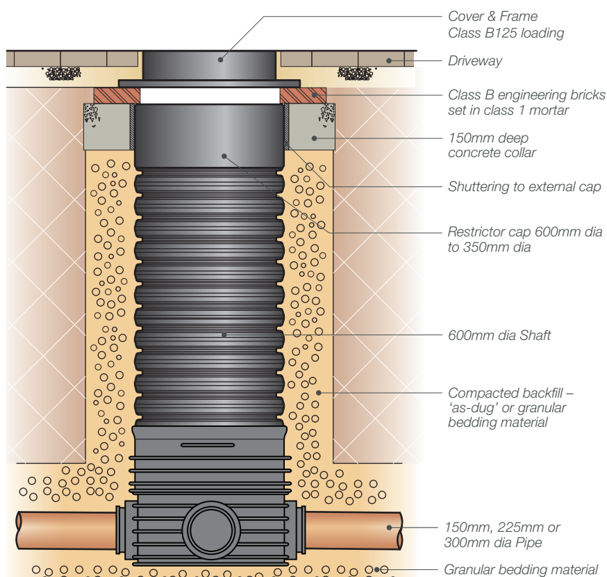
Fig. 34 – Typical installation domestic detail: Range 600 Inspection Chamber. Type 3
