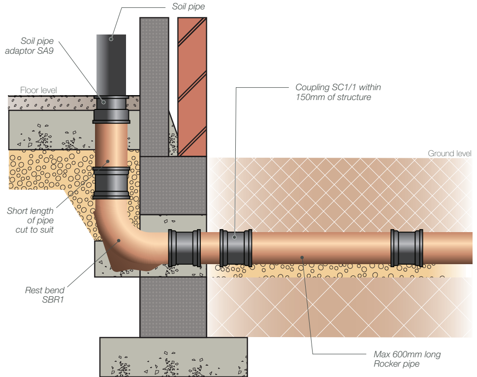
Fig. 17 – Connection of 110mm internal rainwater – soil pipe
