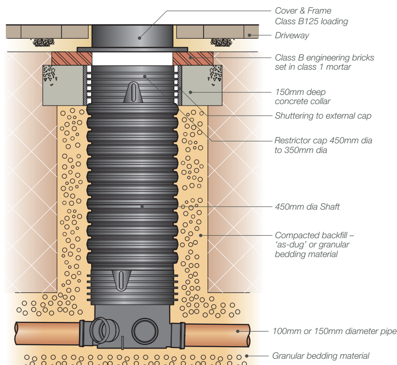
Fig. 31 – Typical installation domestic detail: Range 450 Inspection Chamber. Type 3
