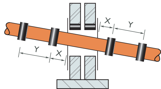
b. Pipe through lintelled opening
