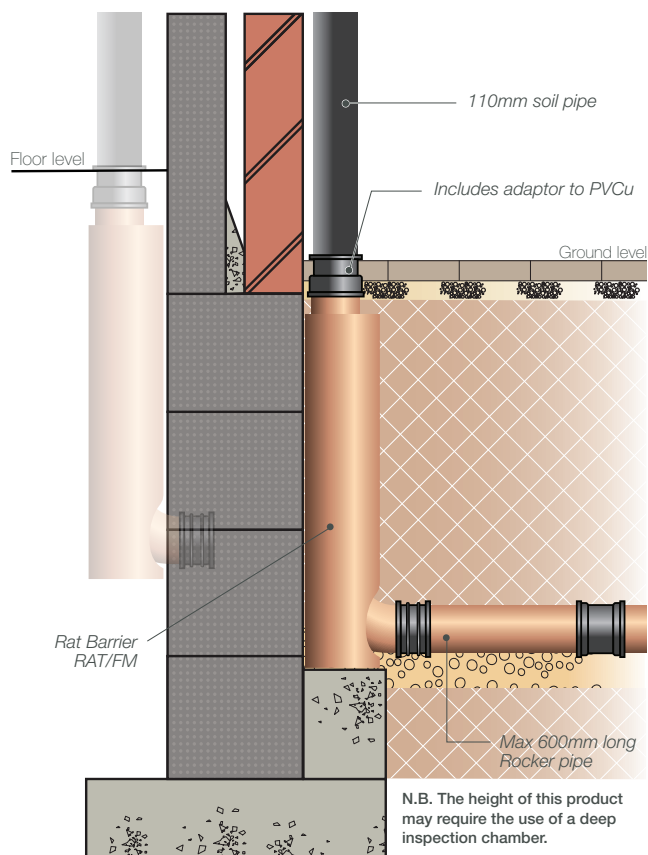
Fig. 19 – Rat Barrier installation
