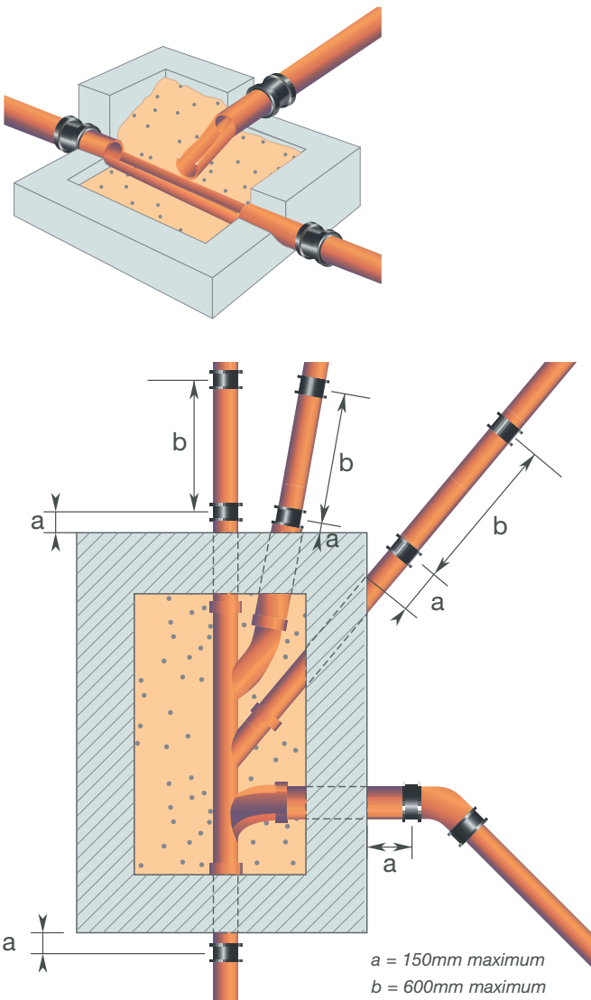
Fig. 37 – Manhole construction with flexible joints
