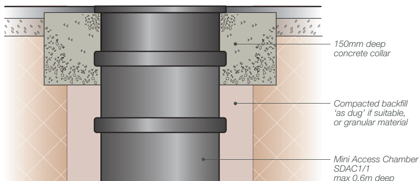
Fig. 27 – Installation detail – domestic paths/patios
