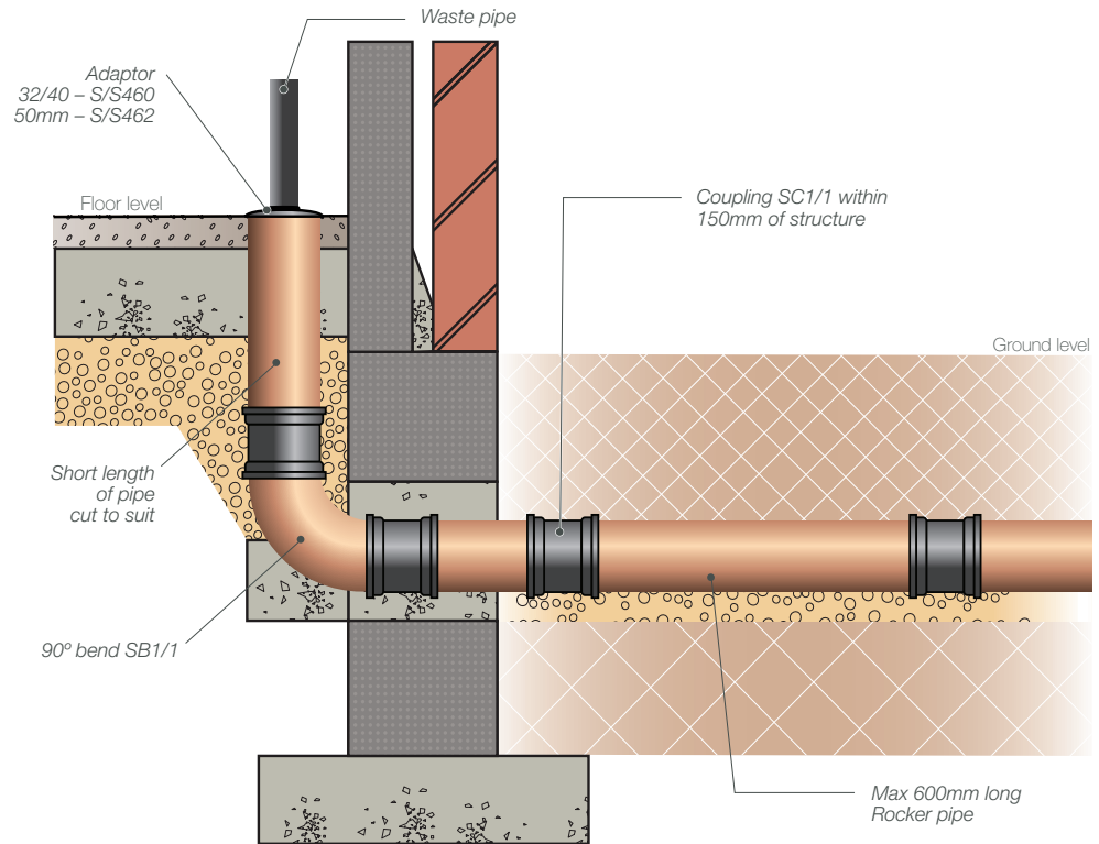
Fig. 15 – Connection of internal waste pipe
