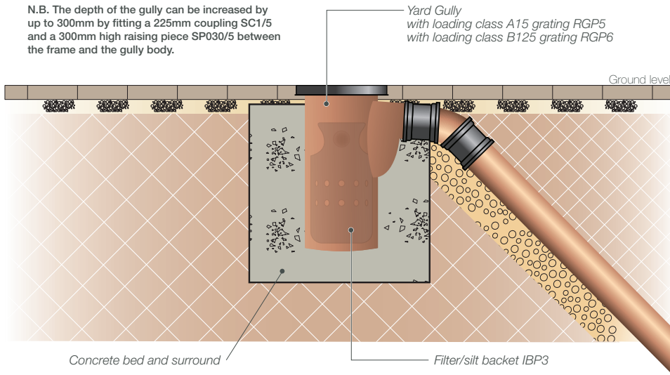
Fig. 24 – Yard Gully
