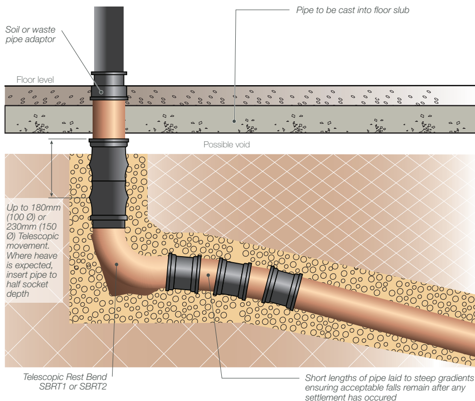
Fig. 18 – Telescopic Rest Bend installation
