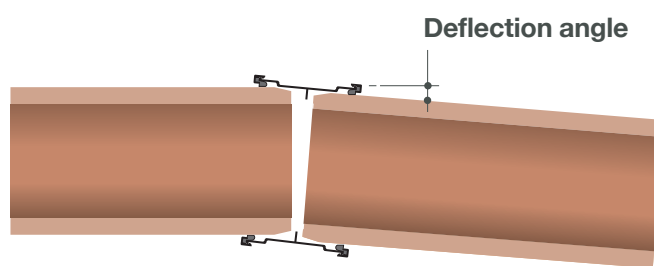
SuperSleve joint
