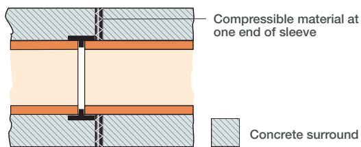
Fig. 12 – Protection of a shallow pipeline
