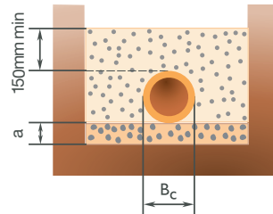
Class F Bedding Factor 1.9
