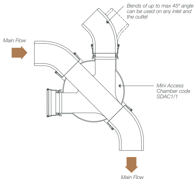
Fig. 26 – Installation detail – domestic gardens
