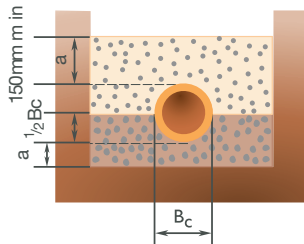
Class B Bedding Factor 2.5
