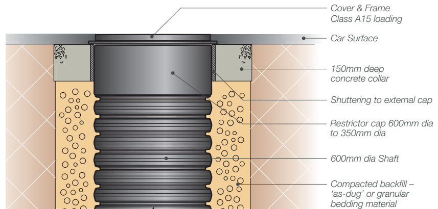
Fig. 35 – Installation detail A15 – domestic gardens and/or areas subject to occasional vehicle loading
