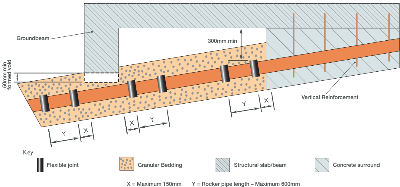
Fig. 11 – Vitrified clay pipeline under typical building slab
