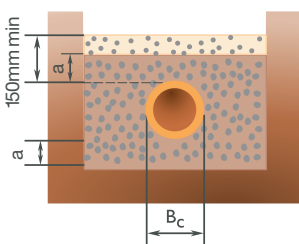
Class S Bedding Factor 2.5
