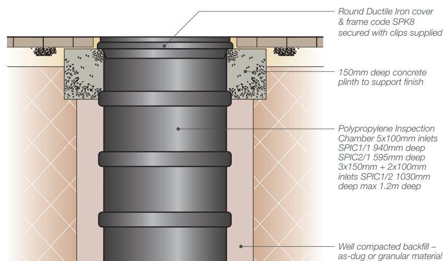
Fig. 29 – Installation detail – domestic paths/patios
