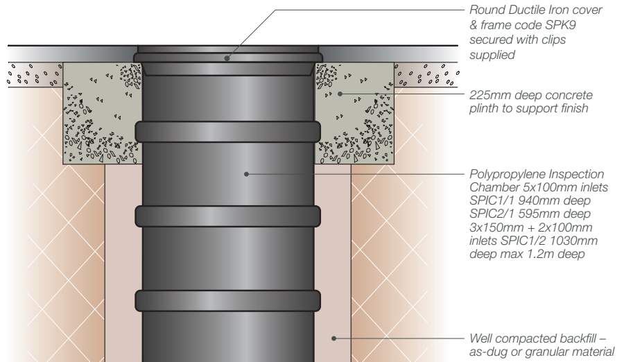
Fig. 30 – Installation detail – domestic driveways
