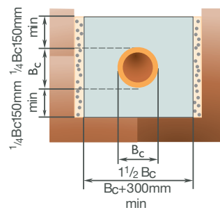
Bedding Factor 4.5
